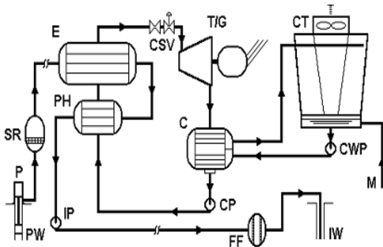
Fig. 2. Flow diagram of basic binary geothermal power plant. PW : production well, P : well head pump, SR : separator, E : evaporator, PH : pre-heater, CSV : control valve, C : condenser, T/G : turbine and generator, CP: feeding pump, CWP : cooling water pump, CT : cooling tower, M : makeup water and IW : injection well.
