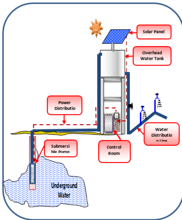
Figure 5: Diagram of Underground water plant
