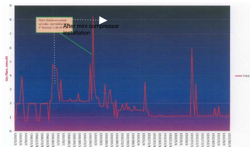
Figure 5. Flare monitoring in Field S before and after installation
