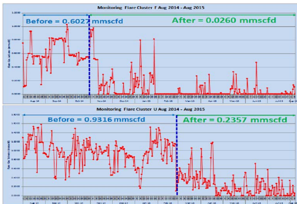
Figure 7. Flare monitoring in Field T before and after installation
