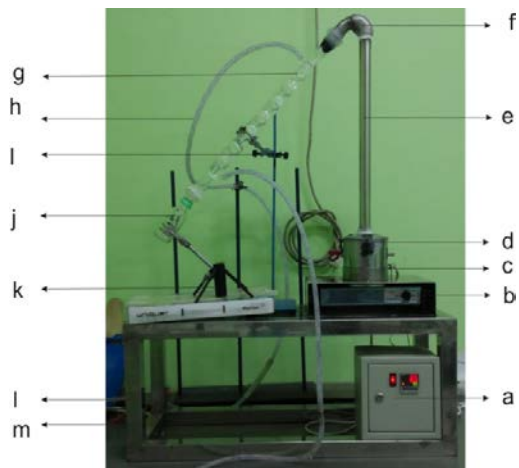
Figure 1. Purification Equipment Laboratory Scale Ethanol
