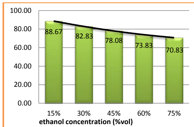
Figure 4. Boiling point of ethanol-water dilutions.
